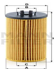
Oil Filter HU 835/1 z EM-10071
